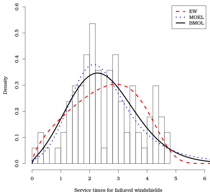
Figure 4: Comparison of the EW, MOEL and BMOL estimated densities for the service times data.
