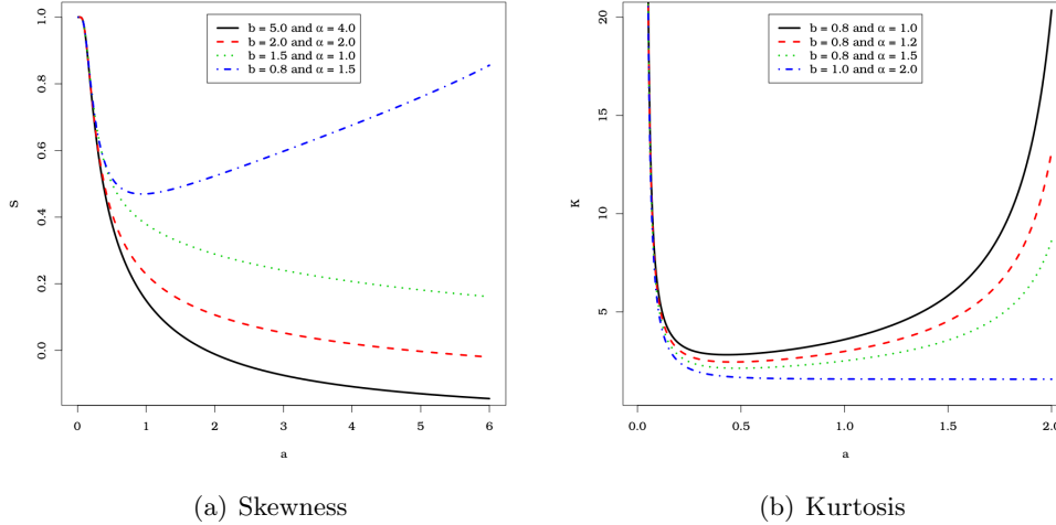
Figure 3: Plots of S of Bowley skewness (5.2) and of K of Moors kurtosis (5.3) measures for selected parameters ( c = 2.0 ).
