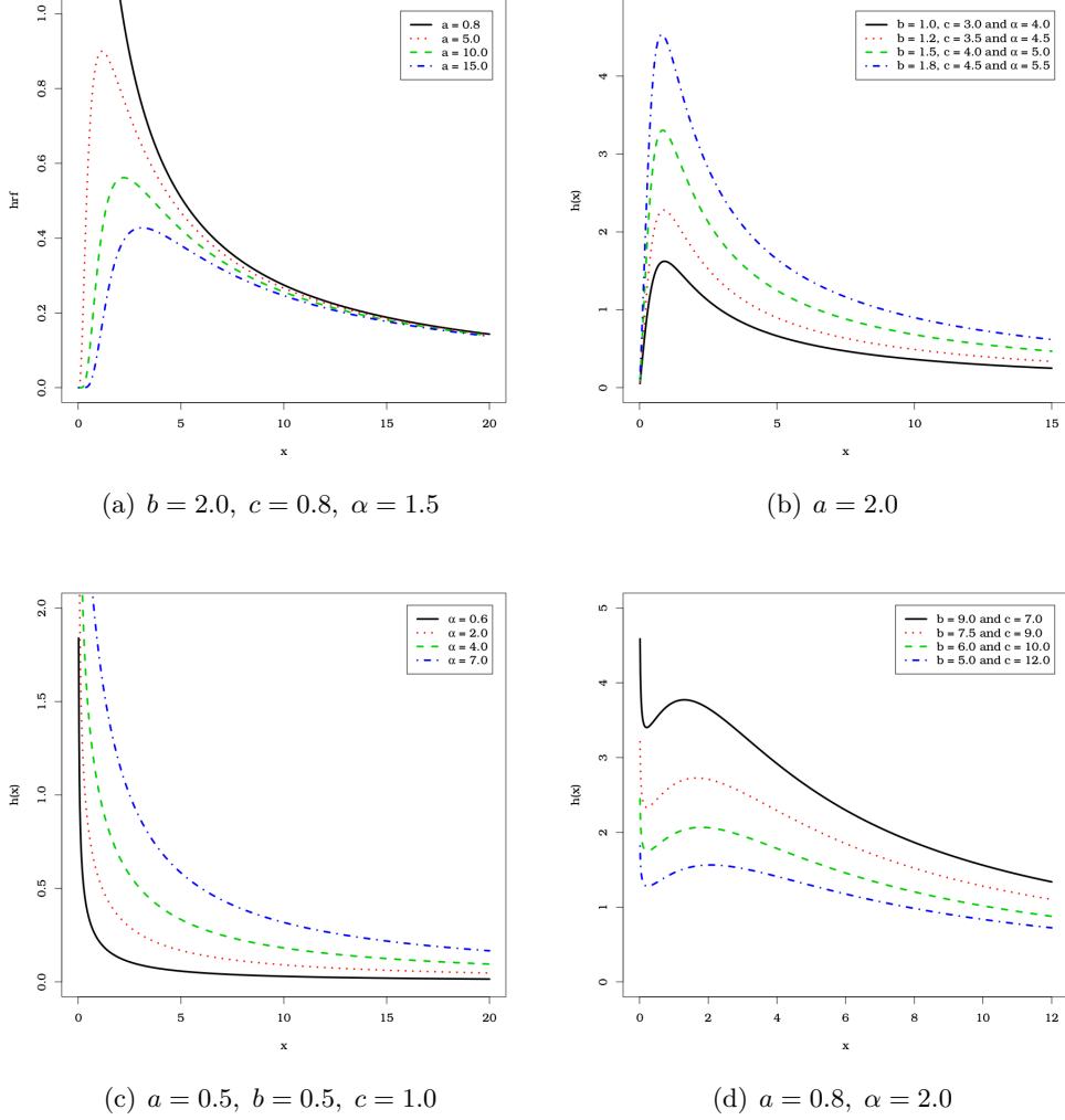
Figure 2: Plots of the hrf (2.10) for selected parameters.
