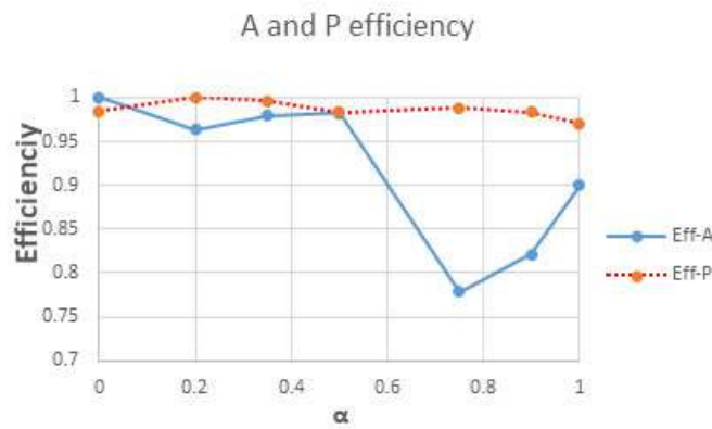
Figure 2: A- and P-efficiencies of AP-optimal designs for different values of \alpha .
