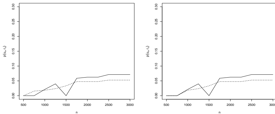
Figure 3: Observed proportions of anti-D (3) ( u_n ) (left) and anti-D (4) ( u_n ) conditions for Uccle data, for \tau = 15 (full line) and \tau = 20 (dashed line), with k_n = \lceil (\log n)^{2.5} \rceil .
