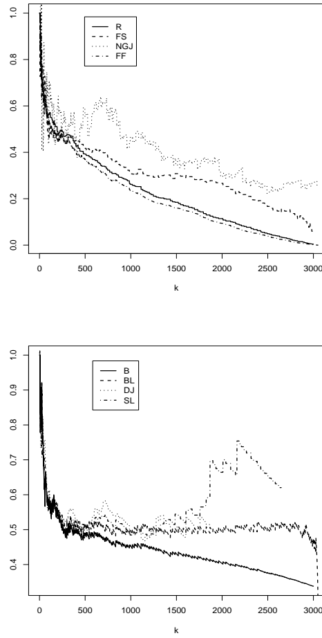
Figure 4: Sample paths of estimators in (2.11) and estimator (3.1) for Uccle data.
