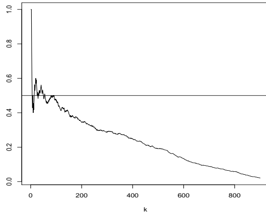
Figure 1: Runs estimates sample path of a moving maximum process, X_i = \max(a_0 Z_i, a_1 Z_{i-1}, a_2 Z_{i-2}) , i \geq 1 , where \{Z_i\}_{i \geq -1} is an i.i.d. unit Fréchet sequence, a_0 = 1/3 , a_1 = 1/6 and a_2 = 1/2 , with run length r = 2 . The horizontal line corresponds to the true value.
