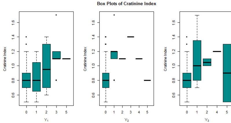
Figure 2: Boxplots of creatinine index versus the number of acute rejections for all time points.
