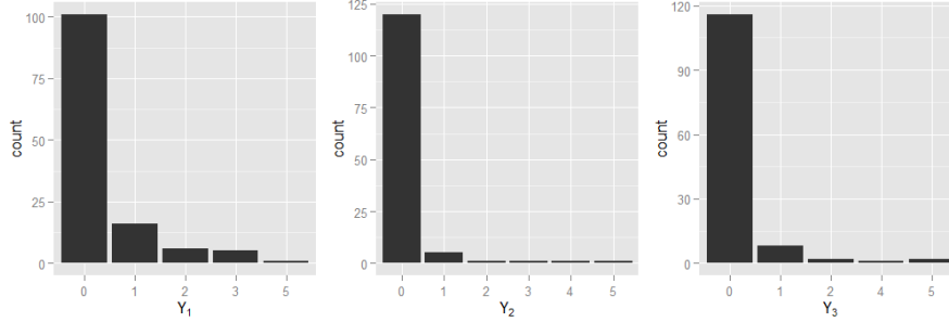
Figure 1: Barcharts of the number of acute rejections for time point at month 4 (first panel), month 8 (middle panel) and month 12 (third panel).
