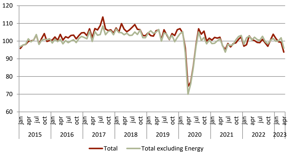
Figure 1. Industrial Production Index, Base 2015=100 Total and excluding Energy
